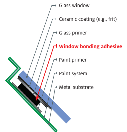
CROSS SECTION OF TRADITIONAL WINDOW BONDING APPLICATION
