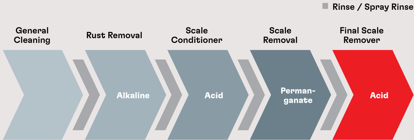
ENGINE OVERHAUL PROCESS
