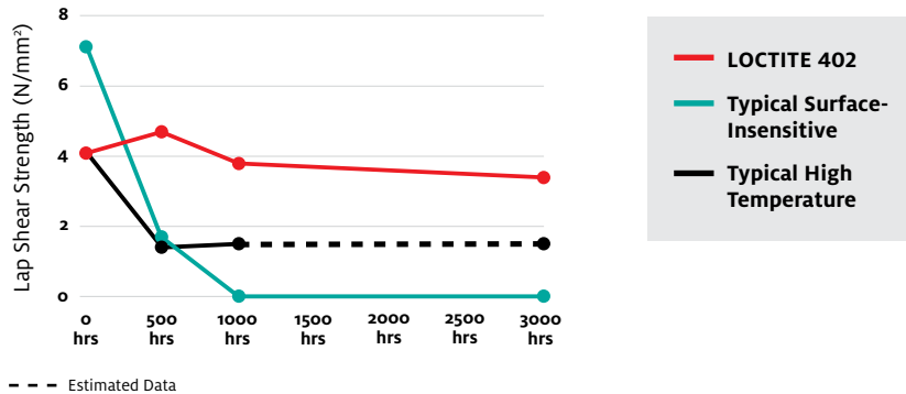
LOCTITE 402 VERSUS TYPICAL INSTANT ADHESIVES: HEAT AGED AT 135°C AND TESTED AT 135°C ON STAINLESS STEEL LAP SHEARS
