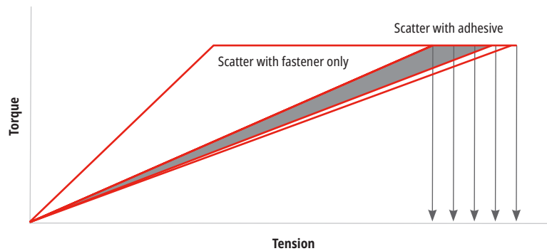
FIGURE 49 Torque-tension scatter: shaded area is with threadlocker, unshaded is without.
