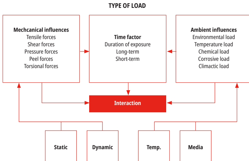
FIGURE 8 Types of loads acting separately or in combination on bonded joints.
