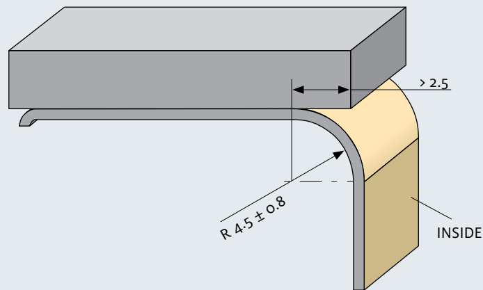
FIGURE 12: RADIUS DESIGN FOR STAMPED PARTS.
