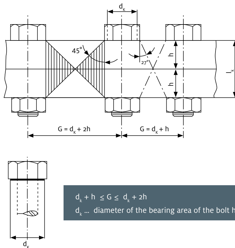
FIGURE 6: PRESSURE CONE ACCORDING TO RÖTSCHER.
