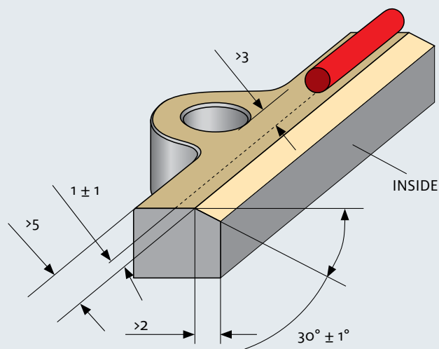
FIGURE 12: CHAMFER DESIGN.
