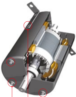
Assembly screws
